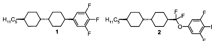
Scheme 1. The liquid crystalline basic structure 1 and its analogue 2 which is extended by a difluorooxymethylene bridge.
